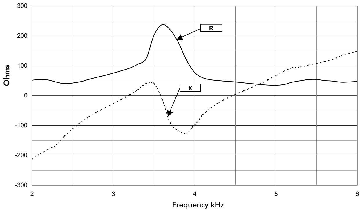
TR-1077A Nominal Resistance, R, and Reactance, X
